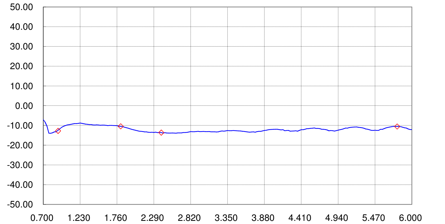
Channel 2 - S11 Return Loss
