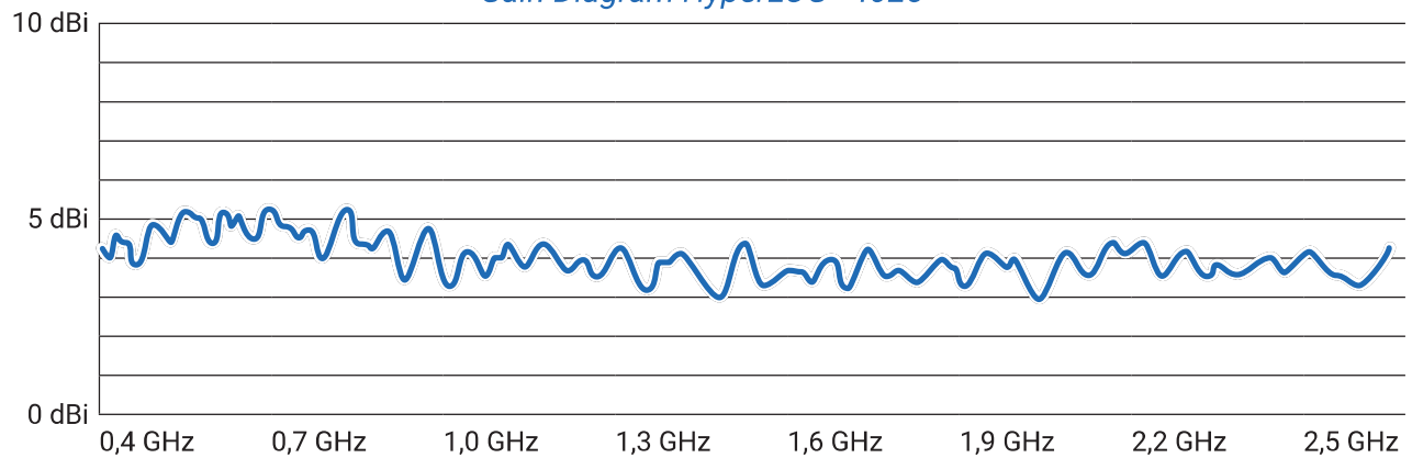
Gain Diagram HyperLOG® 4025
