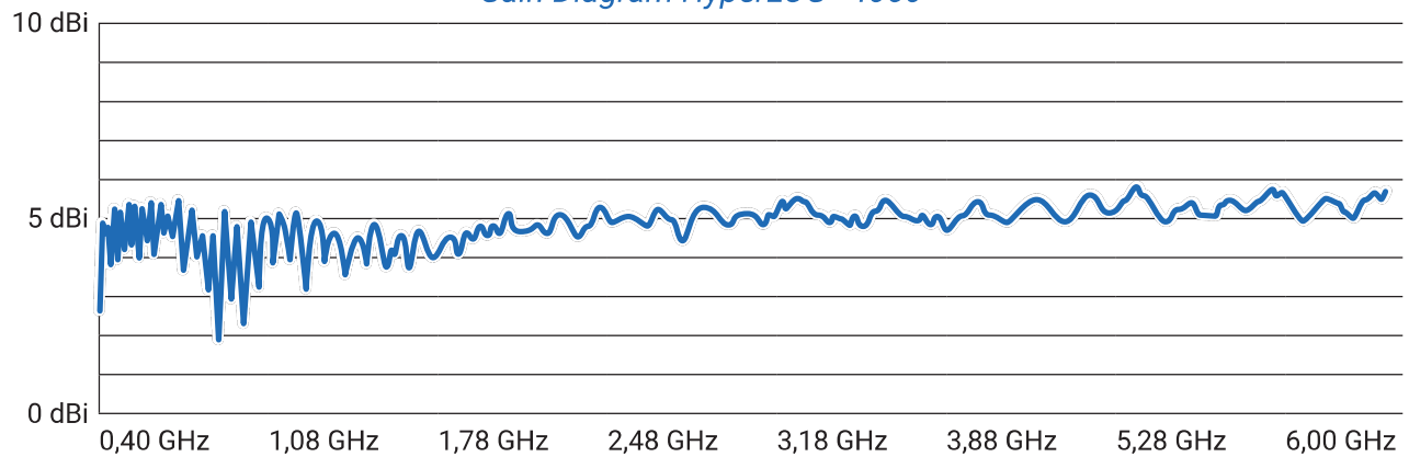
Gain Diagram HyperLOG® 4060
