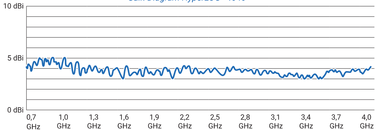
Gain Diagram HyperLOG® 4040
