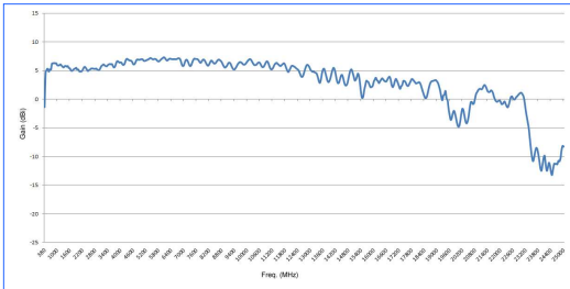
Gain Diagram HyperLOG 30250
