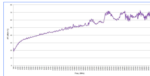
Antenna Factor HyperLOG 30350
