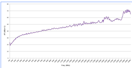
Antenna Factor HyperLOG 30250
