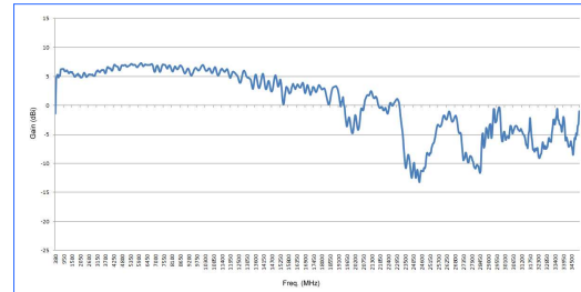
Gain Diagram HyperLOG 30350
