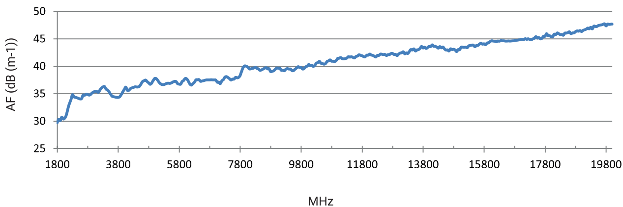
Antenna Factor Diagram HyperLOG® PRO 18200
