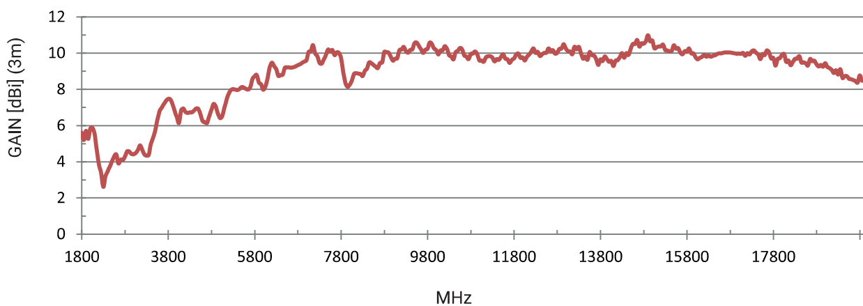
Gain Diagram HyperLOG® PRO 18200
