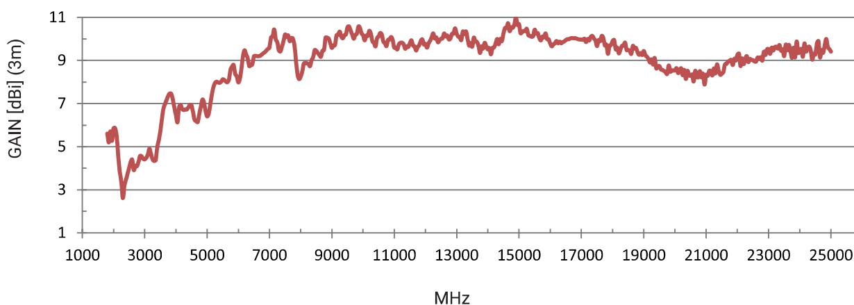
Gain Diagram HyperLOG® PRO 18250
