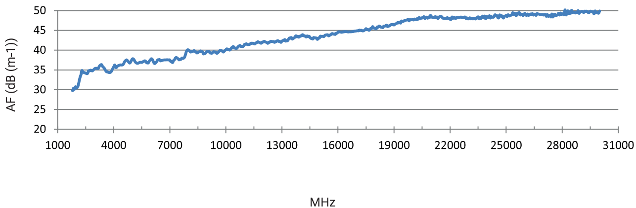
Antenna Factor Diagram HyperLOG® PRO 18300
