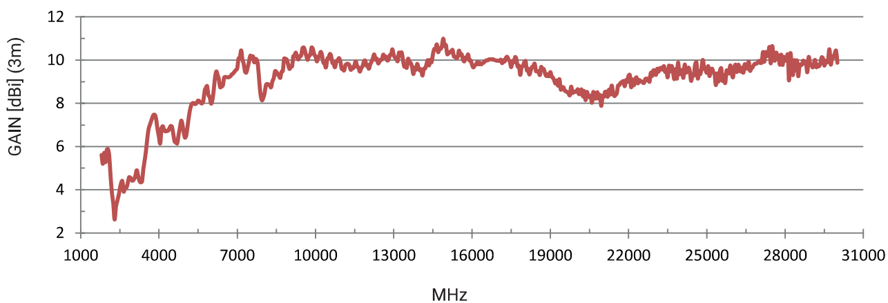
Gain Diagram HyperLOG® PRO 18300
