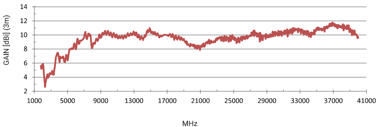
Gain Diagram HyperLOG® PRO 18400
