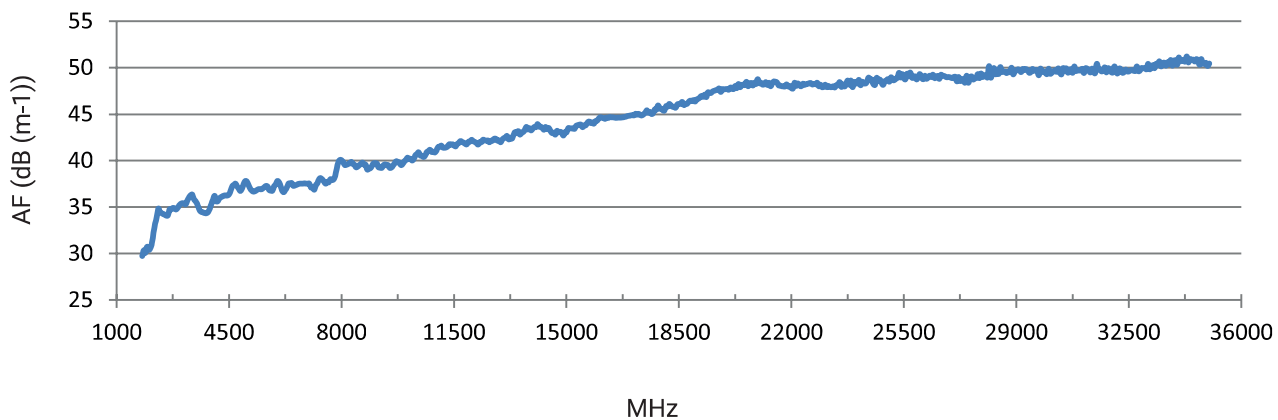
Antenna Factor Diagram HyperLOG® PRO 18350
