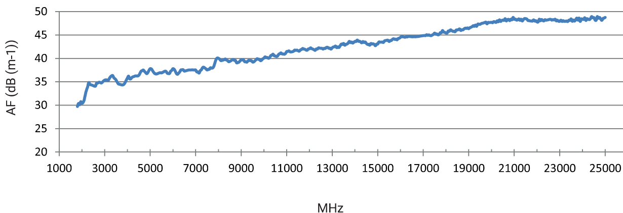
Antenna Factor Diagram HyperLOG® PRO 18250
