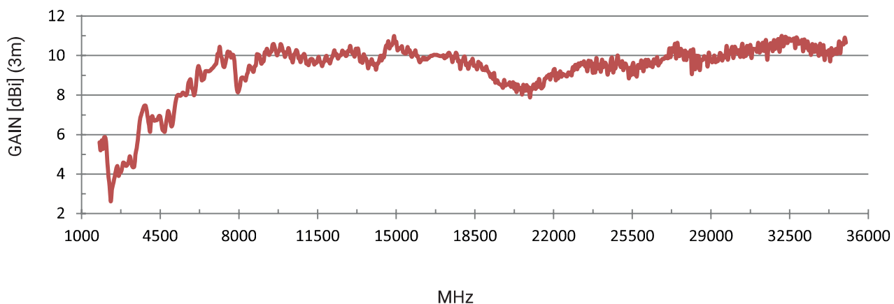
Gain Diagram HyperLOG® PRO 18350
