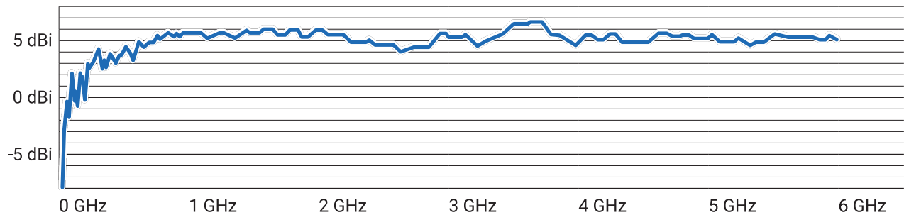
Gain Diagram HyperLOG® 20600 EMI (3 m)
