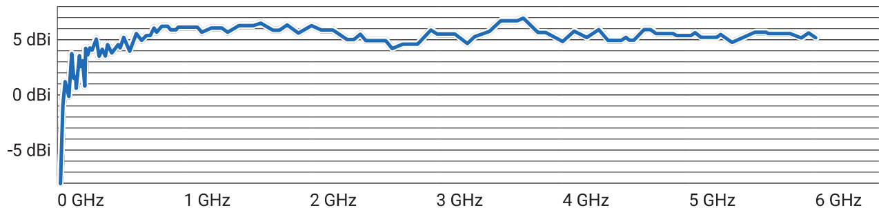
Gain Diagram HyperLOG® 20600 EMI (10 m)
