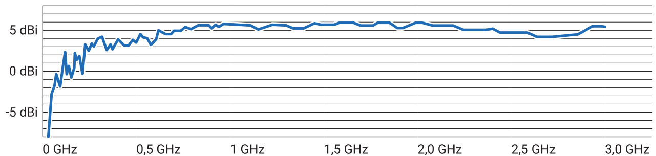
Gain Diagram HyperLOG® 20300 EMI (3 m)
