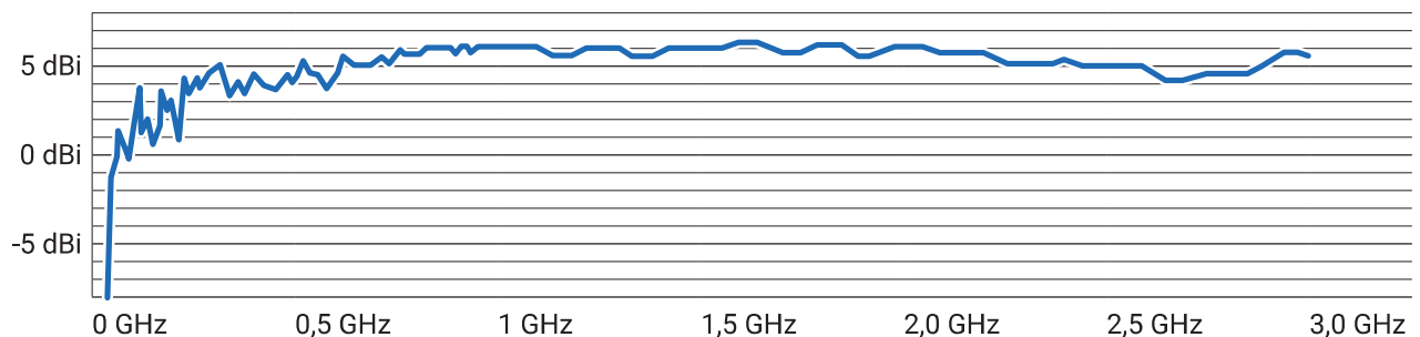
Gain Diagram HyperLOG® 20300 EMI (10 m)
